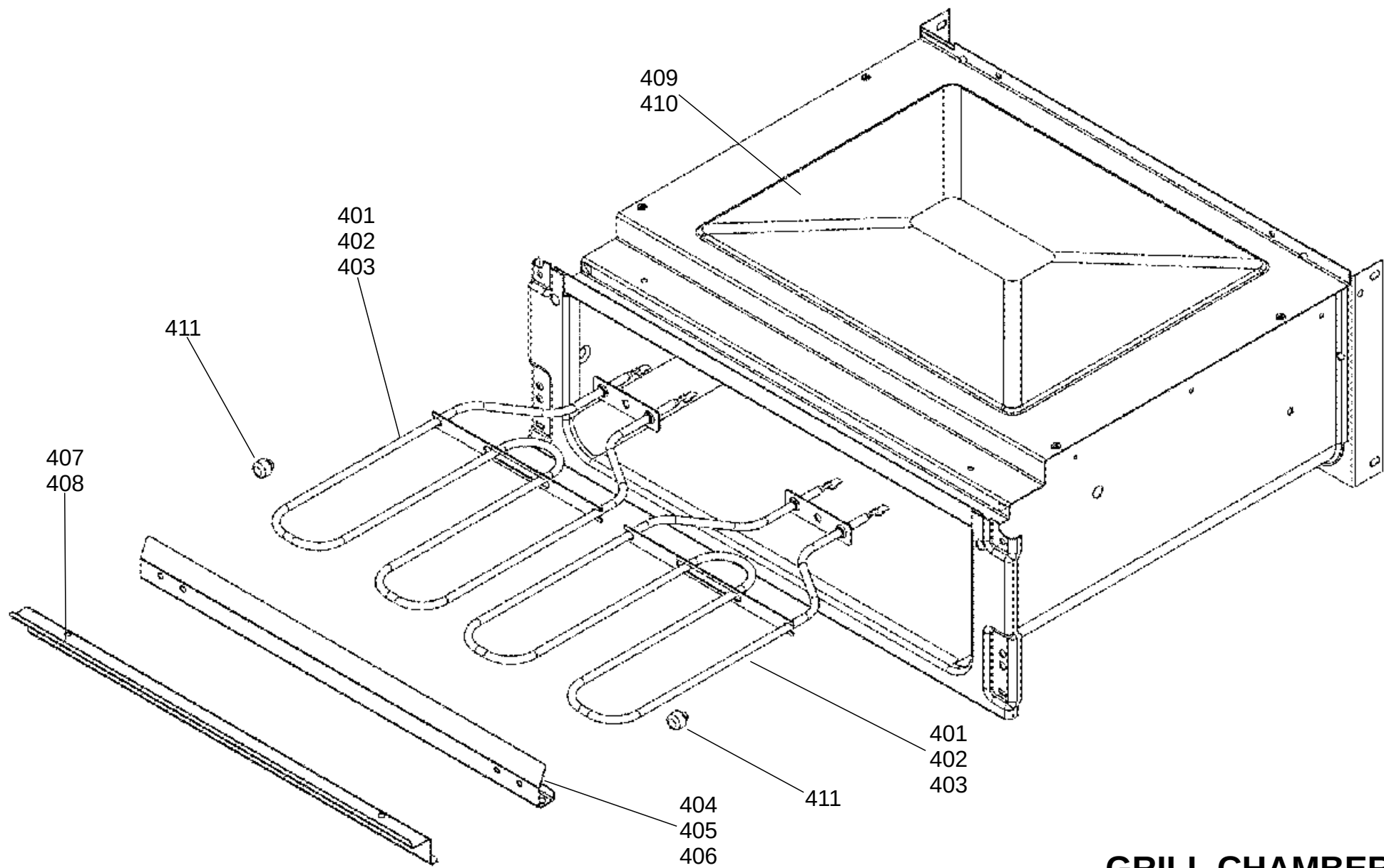
GRILL CHAMBER
